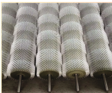
VEG. PEELING ROLLER BRUSH
